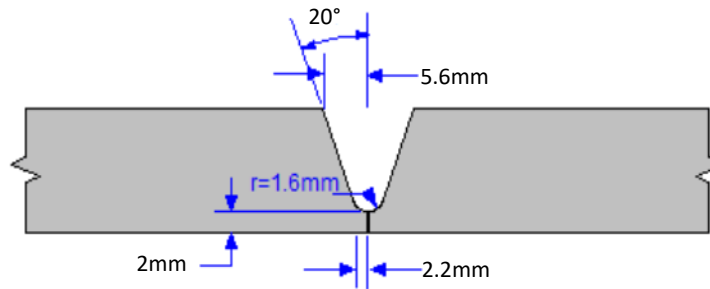
“J” Groove (Fully Automated) Machine Preparation
