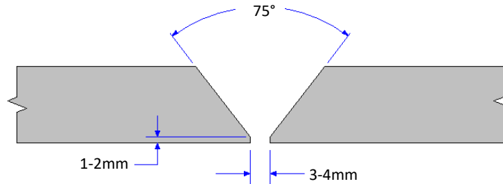
Single Groove (Manual Root) Machine/ Flame Preparation
