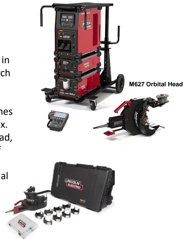
APEX 30S Orbital GTAW System
